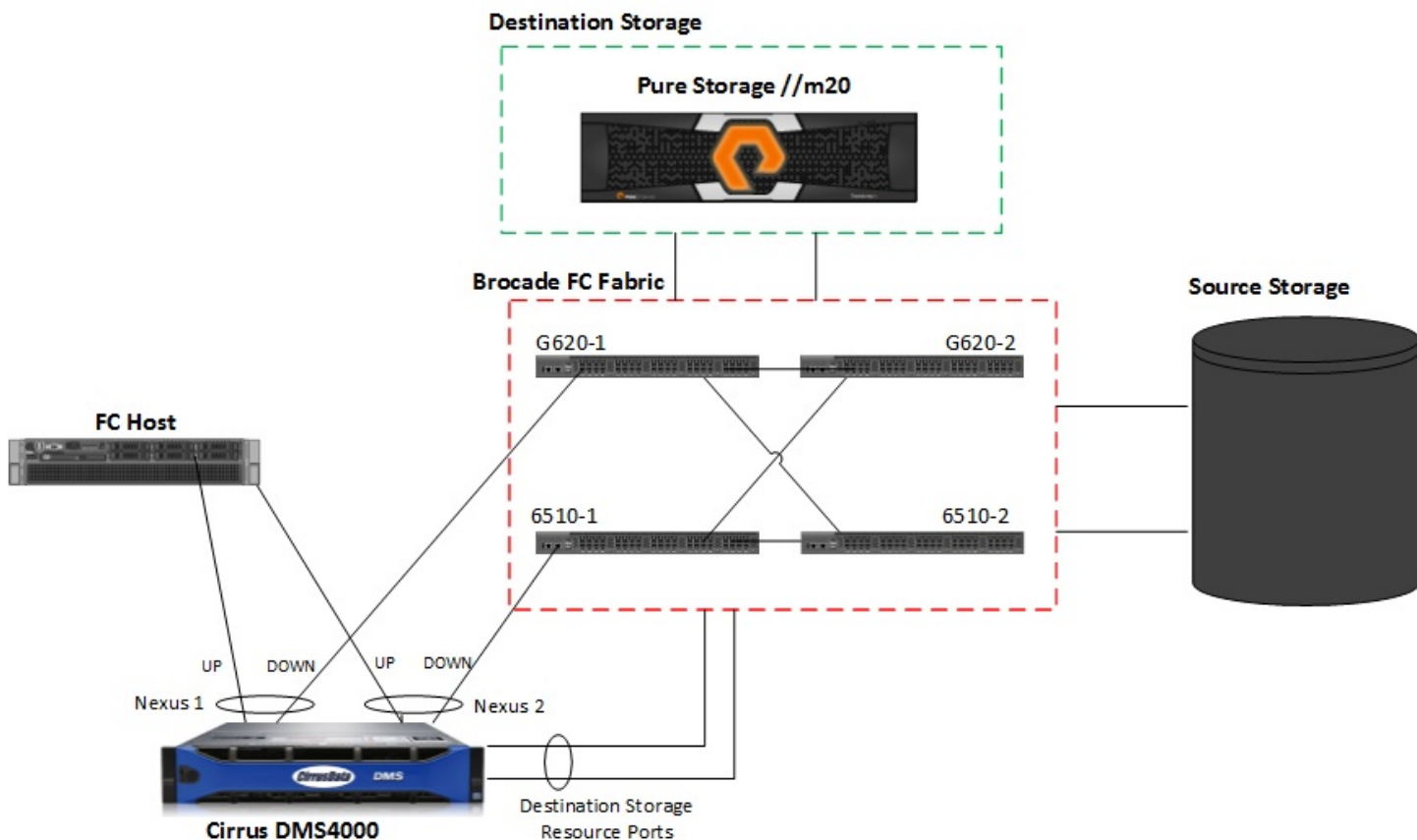
FIGURE 1 Cirrus DMS in Host Side—Physical Intercept Mode
