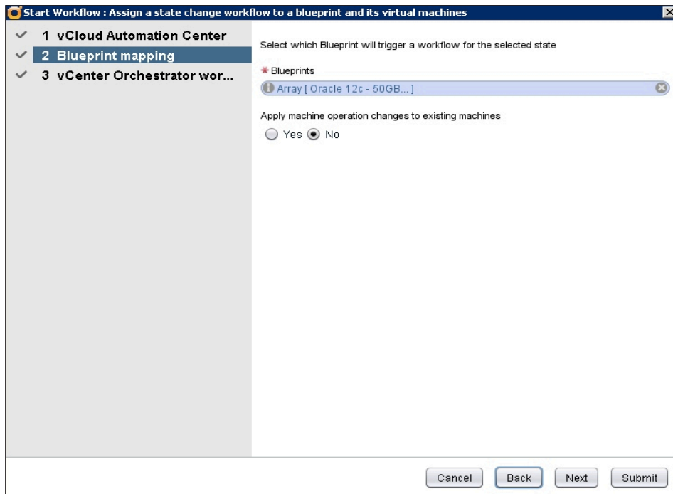
Figure 13: Select vCAC Blueprint to Add vCO Workflow
