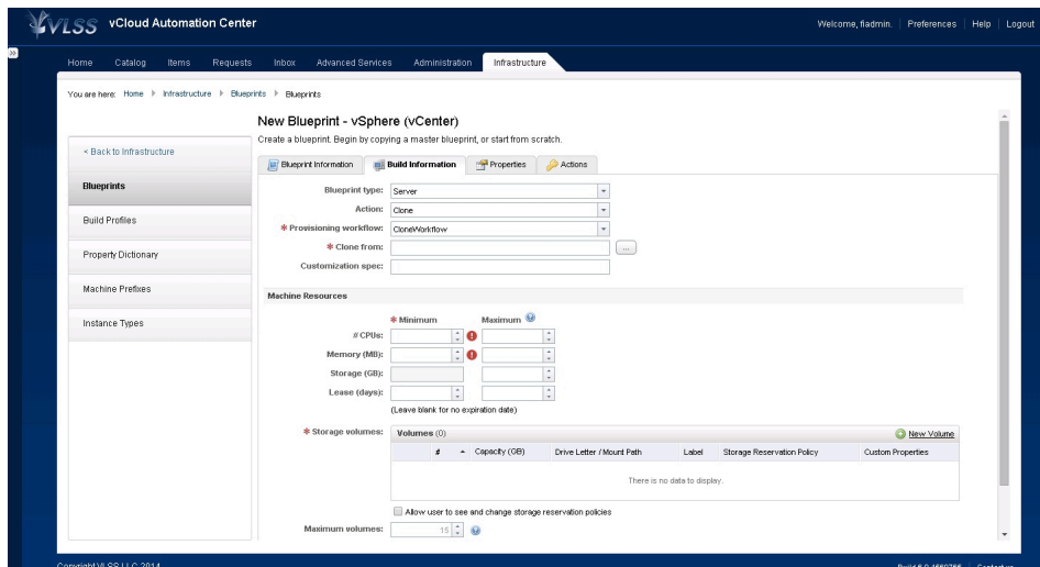
Figure 4: New Blueprint – Set Provisioning Workflow
